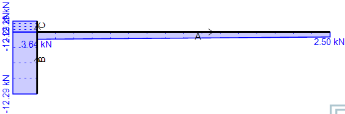
Shear Force Diagram [V]
